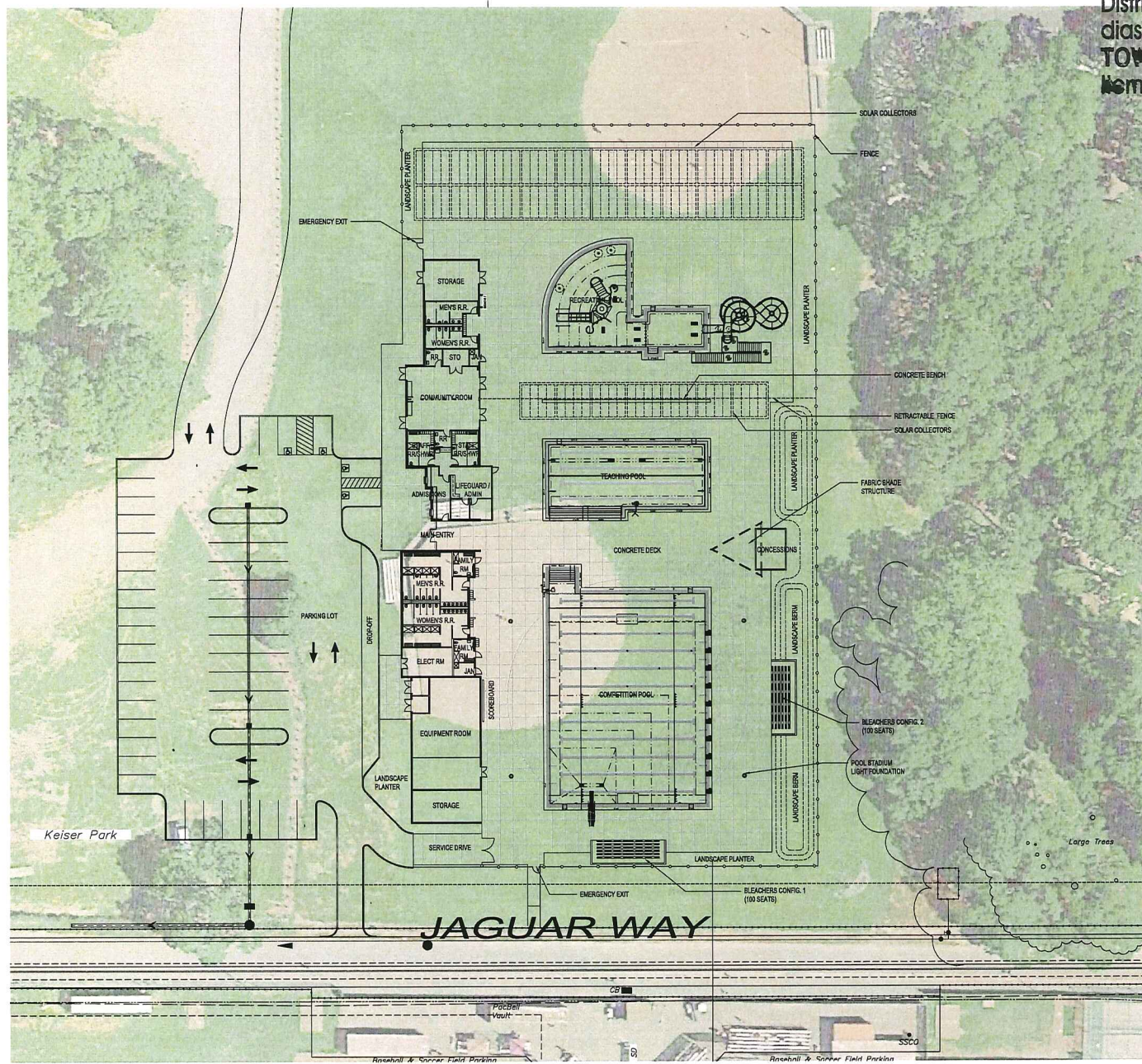
1 SITE PLAN 1"=20'
